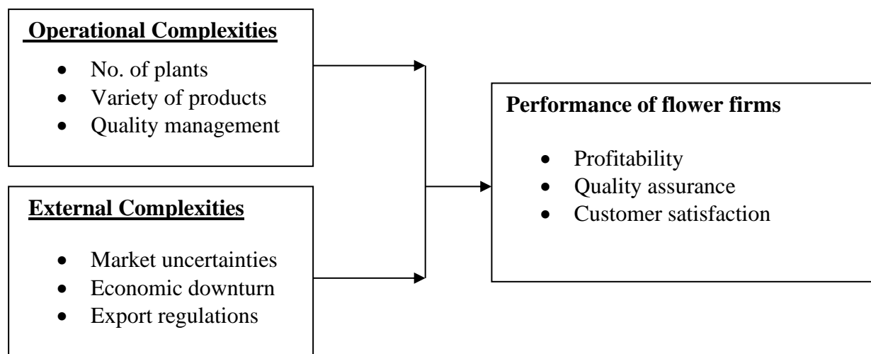
Figure 2.1: Conceptual Framework
